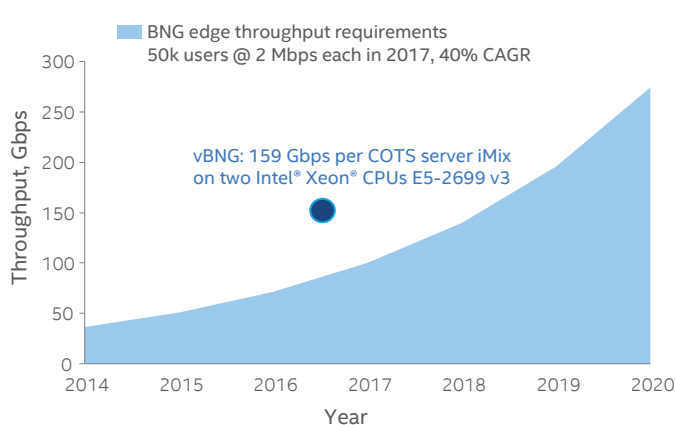
Figure 12. Edge BNG requirements vs NFV performance 17
