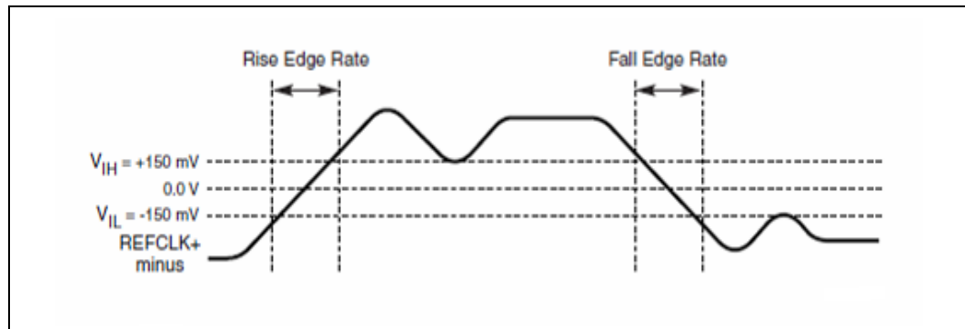
Figure 2-18. Differential Clock Measurement Points for Rise and Fall time
