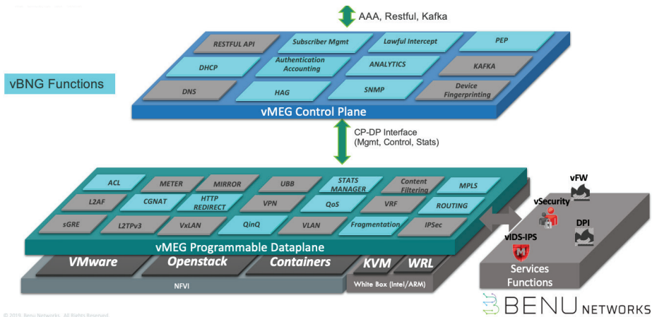
Figure 2. vBNG Functions
